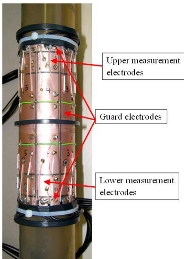
Fig. 1 ECT sensor
