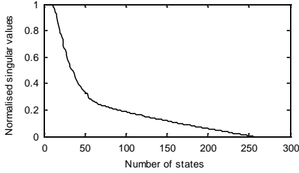
Fig. 3: Normalized singular values for T1
