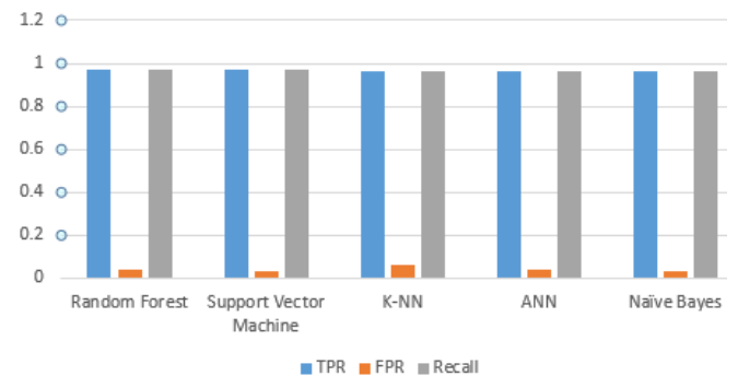
Figure 17 TPR, FPR and Recall
