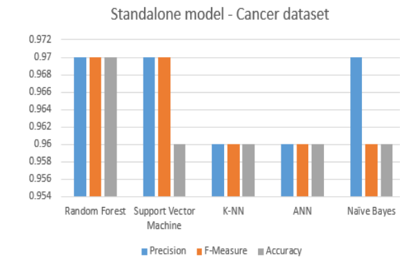
Figure 18 Precision, F-Measure and Accuracy
