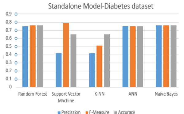
Figure 14 Precision, F-Measure and Accuracy
