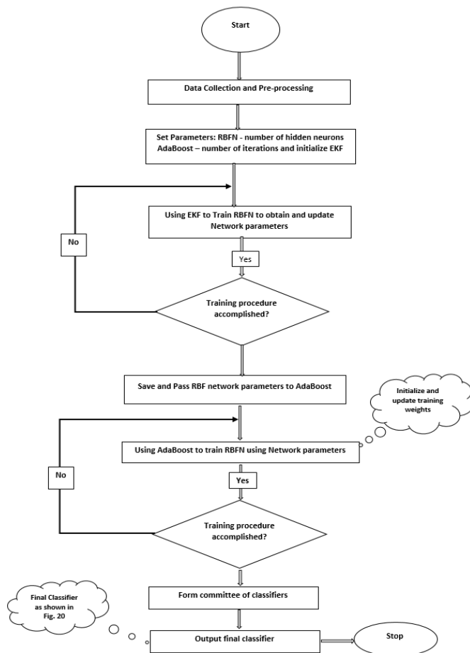
Figure 9 The Architectural flowchart of the proposed EKF-RBFN-AdaBoost Model
