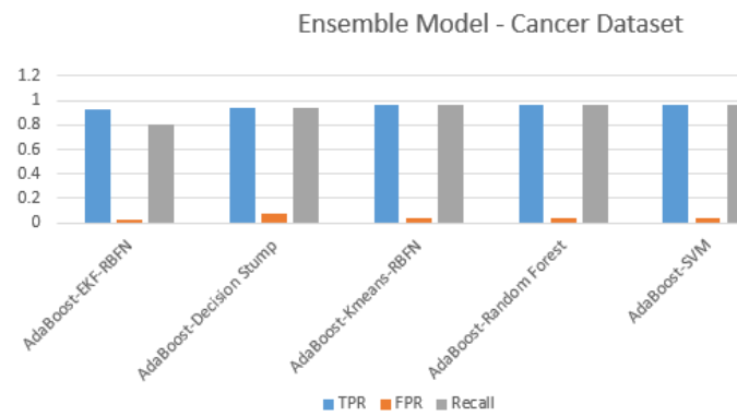
Figure 15 TPR, FPR and Recall
