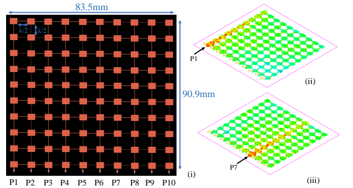
Fig. 4. A planar 10/10 array antenna for 5G mMIMO communication, i) geometric view, ii) P1 radiating view, iii) P7 radiating view.
