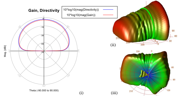
Fig. 9. i) Gain and directivity polar plots of the P1 linear array in the 10x10 MPA array, ii) azimuth and elevation radiating view of the P1 linear array.
