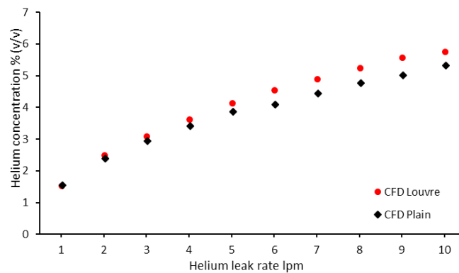
Figure 13 Comparison of CFD plain and louvre vent data at frame sensor 4
