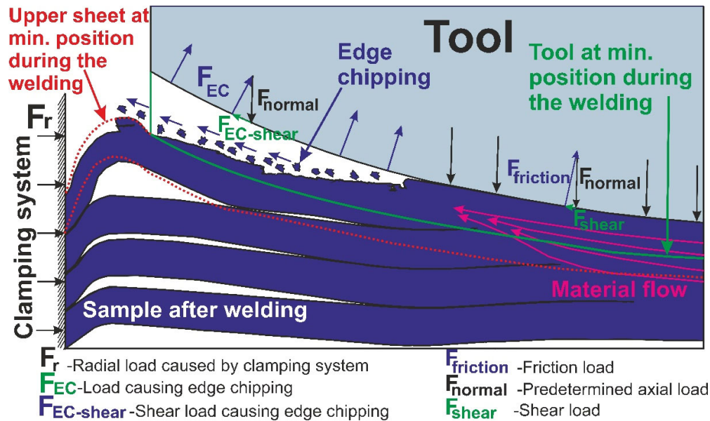
Figure 5. Schematic of the edge-chipping effect.
