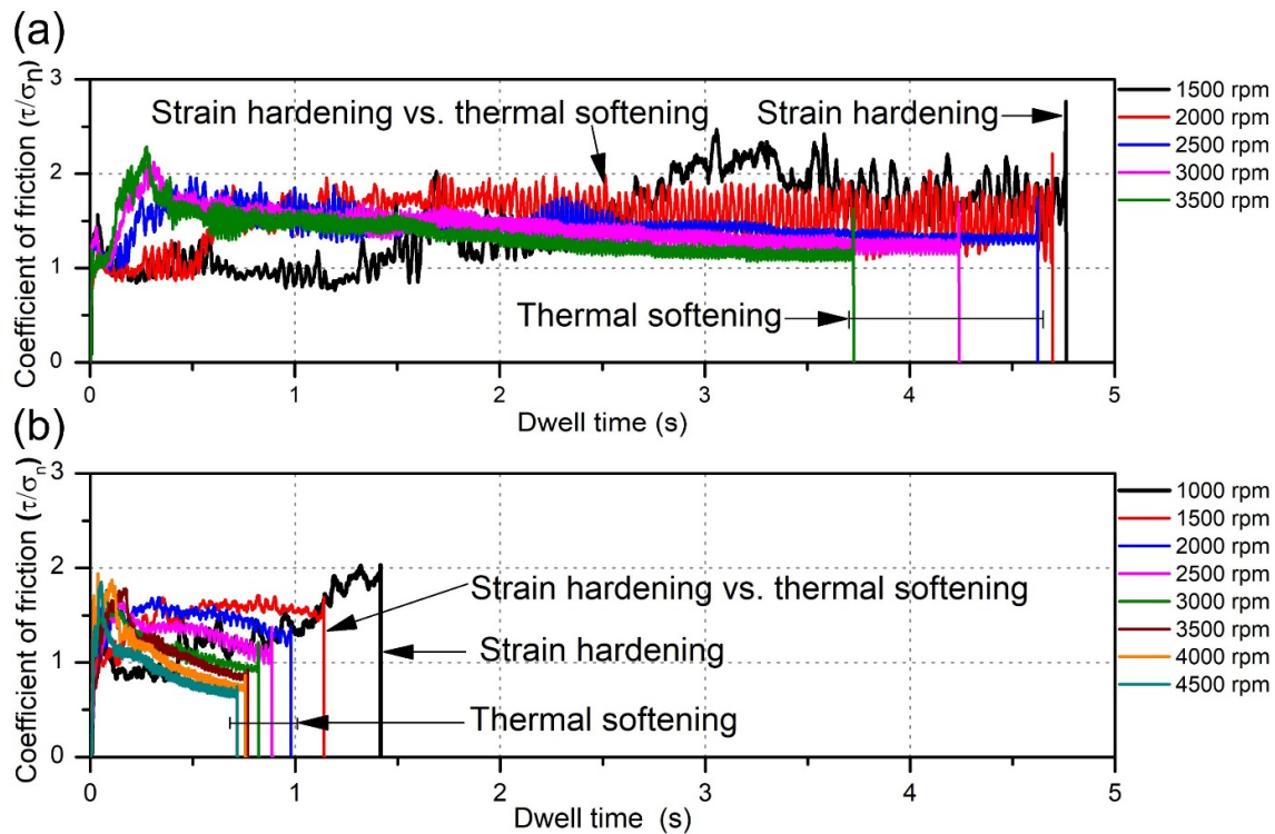
Figure 3. Variation in the coefficient of friction (CoF) over dwell time in: (a) batch I; (b) batch II.
