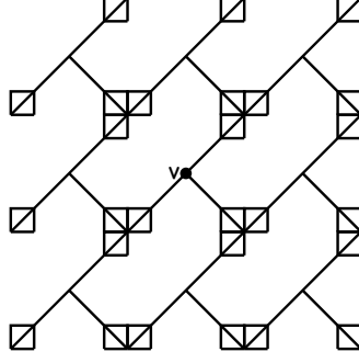
FIGURE 3. Example of a 2-graph on which Theorem 5 can be applied when k = 2 .
