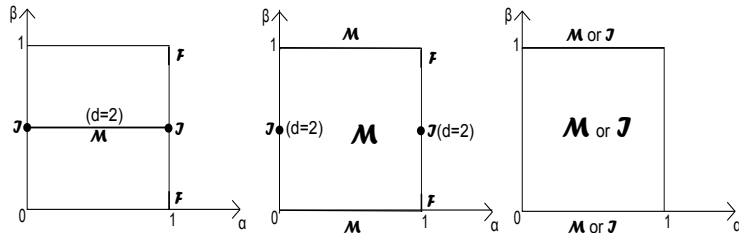
FIGURE 6. Graphical visualization of the conclusions. The panel on the left describes the main results in the literature for the stochastic Ising models at zero-temperature on the graph \mathbb{L}_d . Notice that the case of \gamma = 1/2 holds only for d = 2 . The central panel represents our results for the graphs \Gamma_{\ell, m}(\mathbb{L}_d) . The panel on the right depicts Theorem 2.
