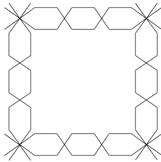
FIGURE 5. Representation of \Gamma_{3,3}(\mathbb{L}_2) .
