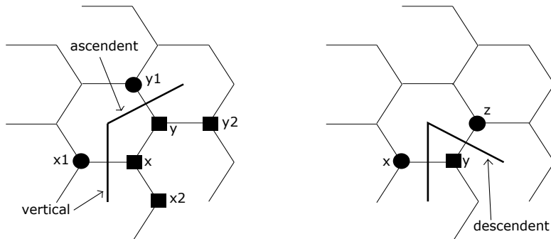
FIGURE 2. The hexagonal lattice with the domain wall \mathcal{D}^H in bold. The squares and the bullets represents spins with opposite signs in the two situations of 2\pi/3 (left panel) and \pi/3 (right panel) angles.
