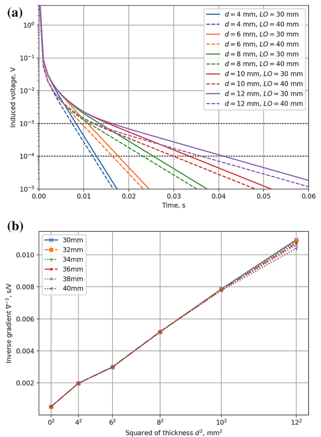
Fig. 1 (a) Simulated PEC signals with varying lift-off and sample thickness, and (b) Extracted |\nabla|^{-1} corresponding to different lift-offs and thicknesses
