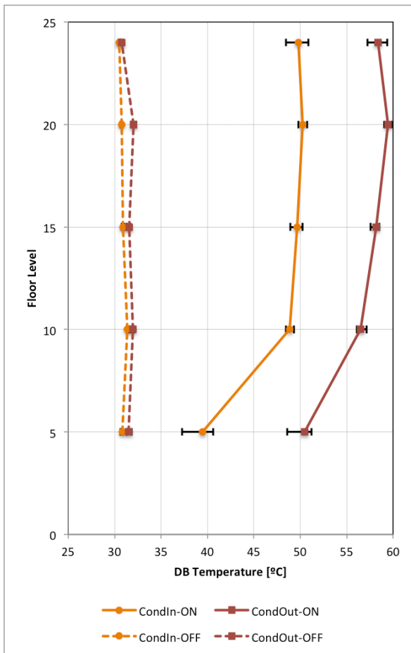
Figure 7. Condenser air temperature distribution, on-coil and off-coil temperature: OFF vs. ON
