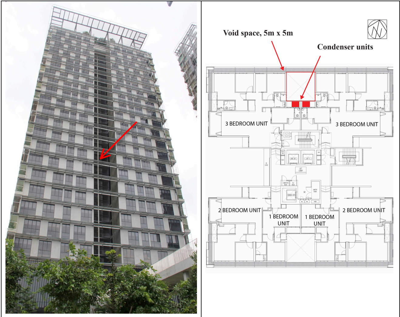
Figure 2. Kent Vale II building with the studied void space - photo and plan.
