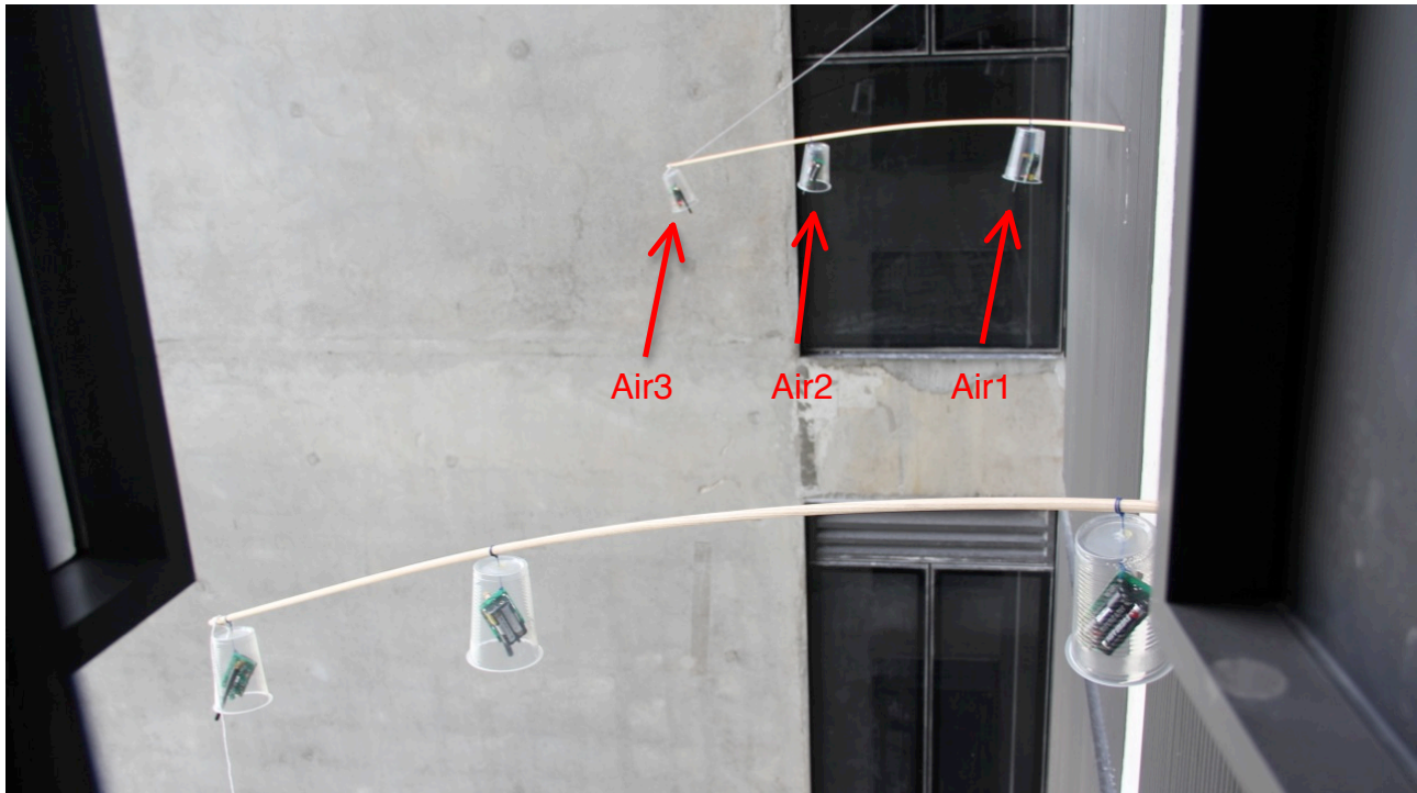
Figure 4. Measurement setup, wireless sensors (Air1, Air2, Air3) placed in void space. At approximate 0, 1 and 2 m.
