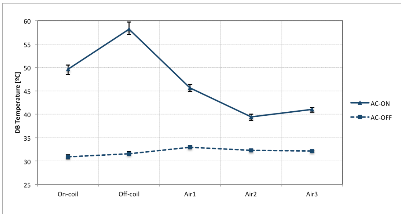
Figure 6. Horizontal temperature distribution on level 15 before and after condenser unit and in void space, separated by louvers.
