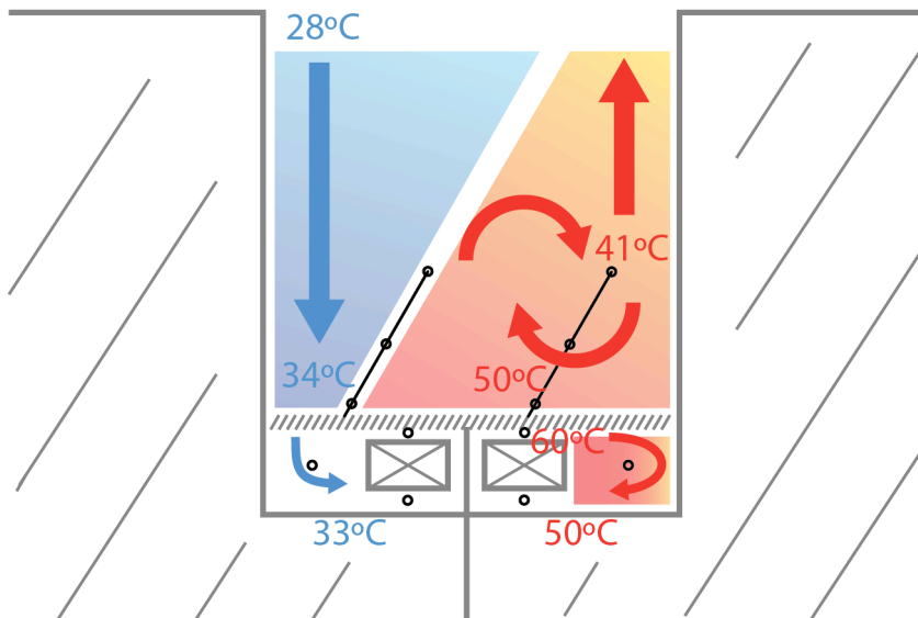
Figure 8. Conceptualisation of horizontal temperature distribution with indicated airflows on level 20.
