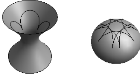
Figure 2: Salkowski curves lying on quadrics. The left one has m = 0.42 and the right has m = 1.0 .
