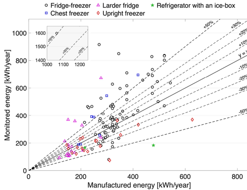
Figure 1. Energy used in the home versus energy claimed by manufacturers.
