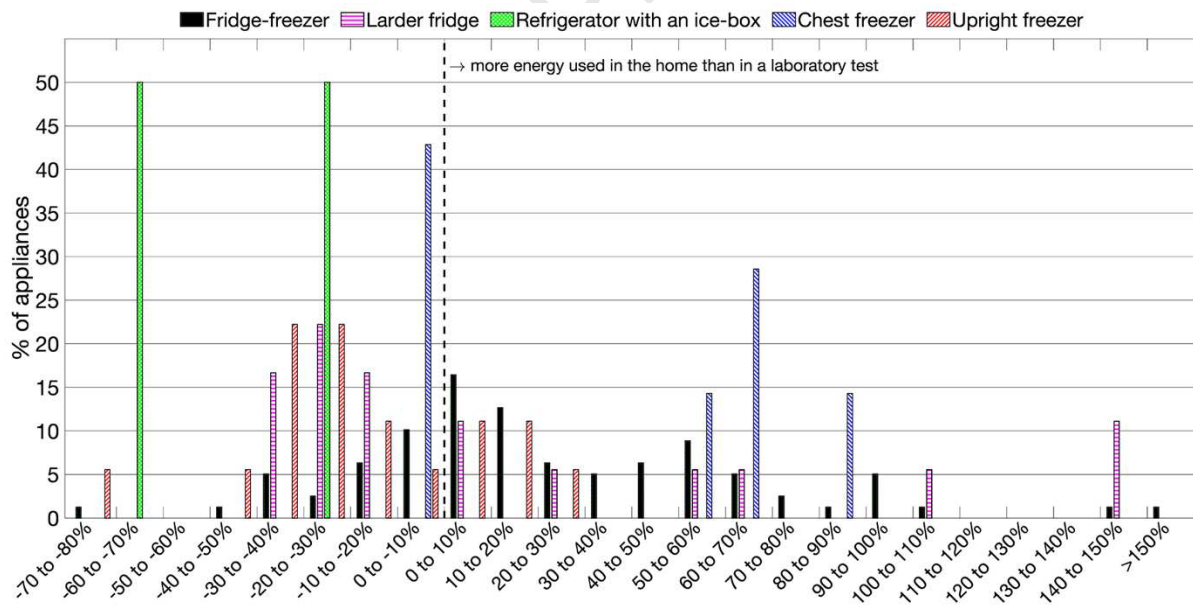
Figure 2. Percentage difference in energy used in the home compared to energy claimed by manufacturer.
