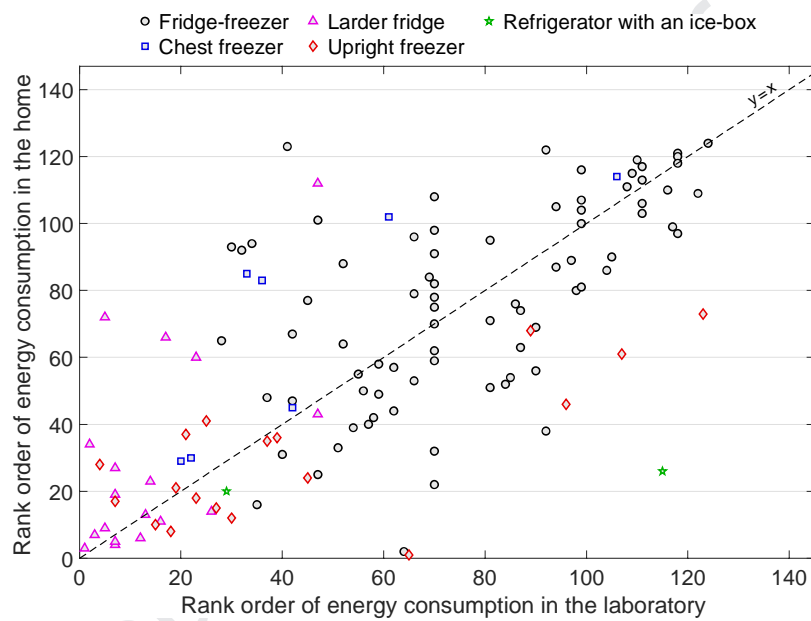
Figure 3. Ascending rank order of energy used by appliances in the home and in the laboratory.
