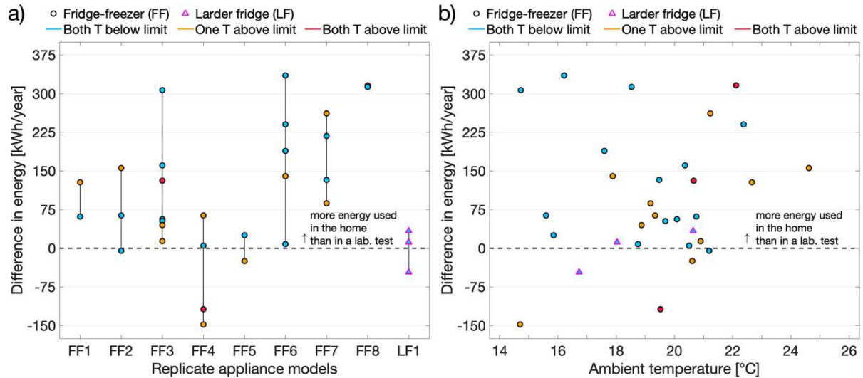
Figure 4. a) Difference in energy used by the same appliance model in different households. b) Difference in energy used plotted as a function of ambient temperature. Inside appliance temperature indicated by colour of data point according to the recommended limits (4 and -18°C).
