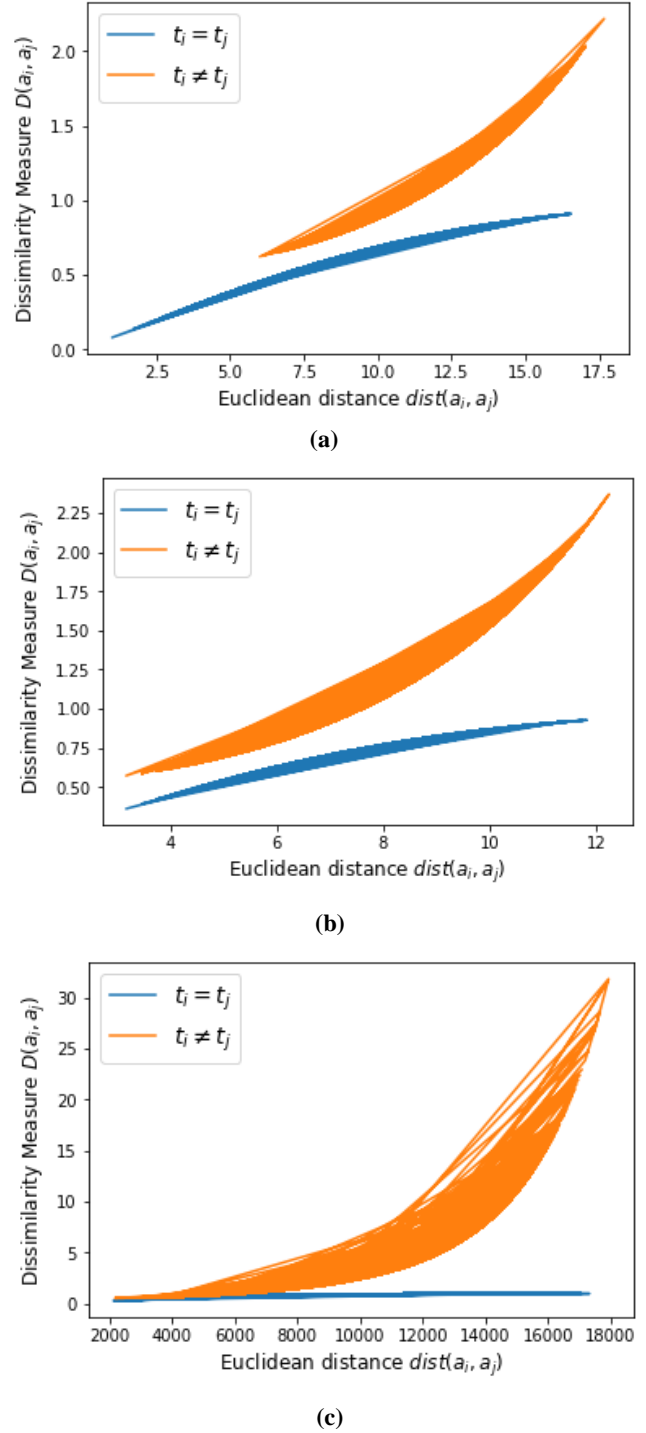
Figure 1. The relationship between Euclidean distance dist(a_i, a_j) and Dissimilarity measure D(a_i, a_j) using MNIST (a), Chest X-ray (b), SEER Breast Cancer (c) datasets.
