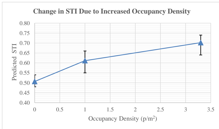
Figure 3 – Predicted change in STI due to Increased Occupancy Density
