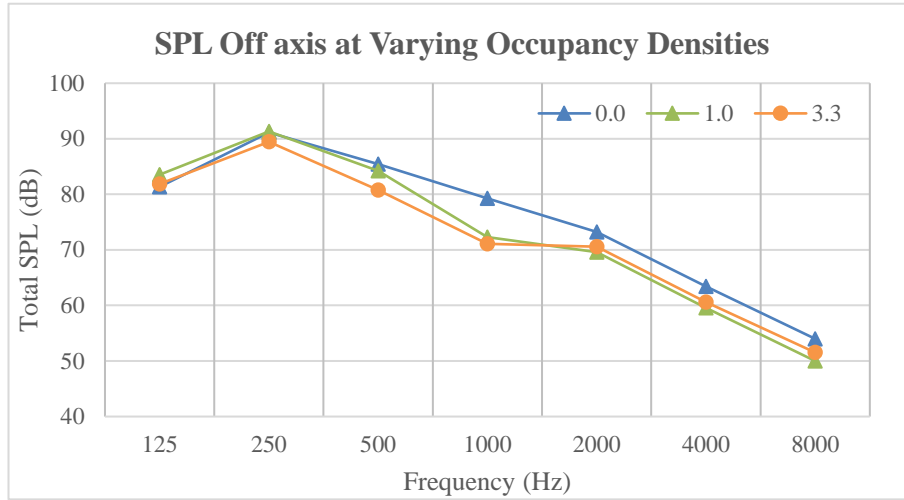
Figure 4 – Octave Band SPL – Off axis
