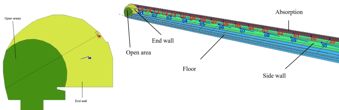
Figure 1 – Cross-section and 3D projection of the platform
