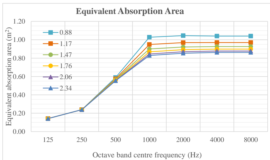
Figure 2 - Calculated absorption area per person at varying occupancy densities
