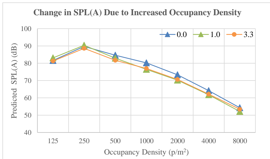
Figure 2 – Predicted SPL Under Varying Occupancy Densities
