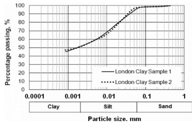
Figure 1. Particle size distribution of London clay
