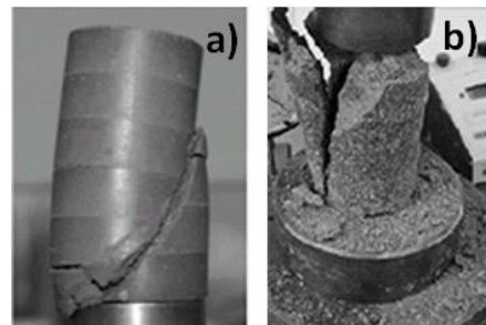
Figure 2. UCS samples a) lime-treated; b) PSA-treated
