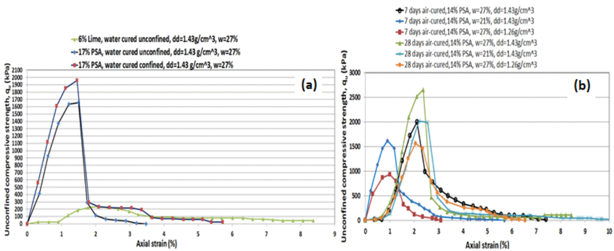
Figure 5. Indicative comparative results of 28-day specimens (a) water-cured specimens; (b) air-cured specimens
