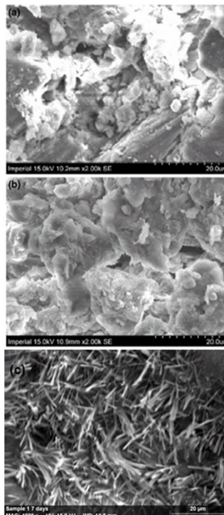
Figure 3. Indicative SEM results: (a) untreated soil; (b) 4% lime-treated soil; (c) 14% PSA-treated soil
