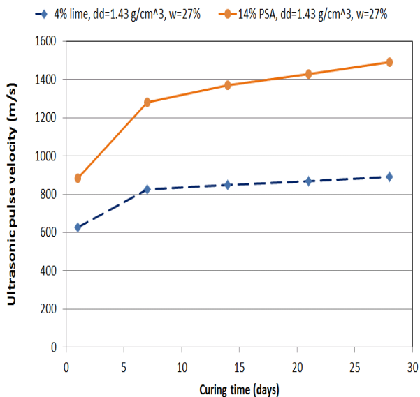
Figure 7. Indicative PUNDIT results (air-cured samples)
