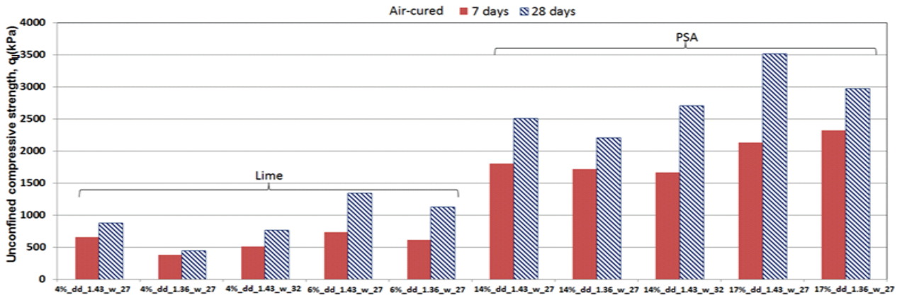
Figure 4. Indicative comparative results of 28-day cured lime-treated vs. PSA-treated specimens
