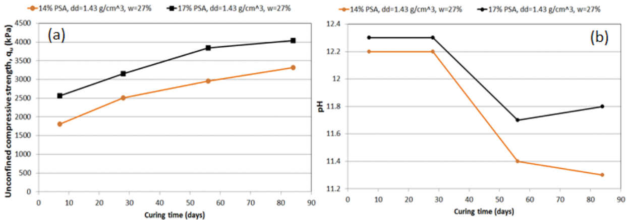
Figure 6. Indicative UCS sample results: (a) evolution of UCS with time; (b) pH of UCS specimens
