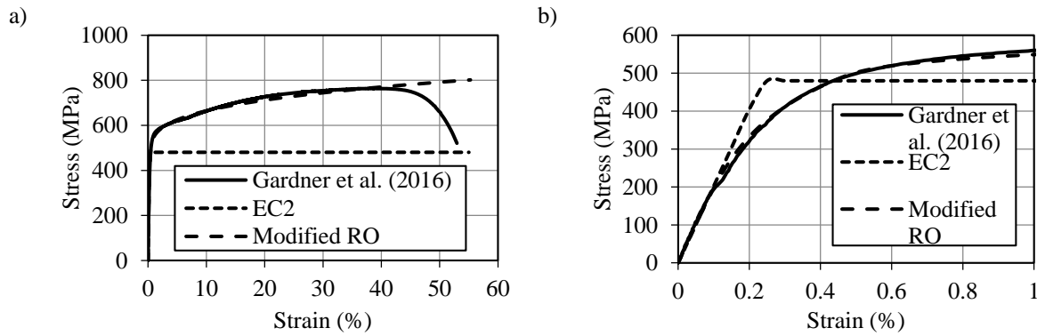
Figure 4. Experimental and design stress-strain curves for grade 1.4311 (a) full curve and (b) more detailed view of the elastic region.
