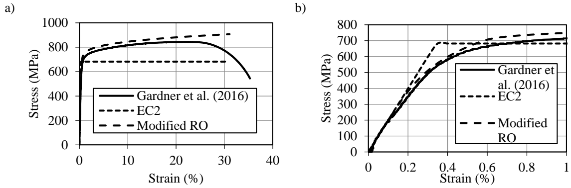
Figure 2. Experimental and design stress-strain curves for grade 1.4162 (a) full curve and (b) more detailed view of the elastic region.
