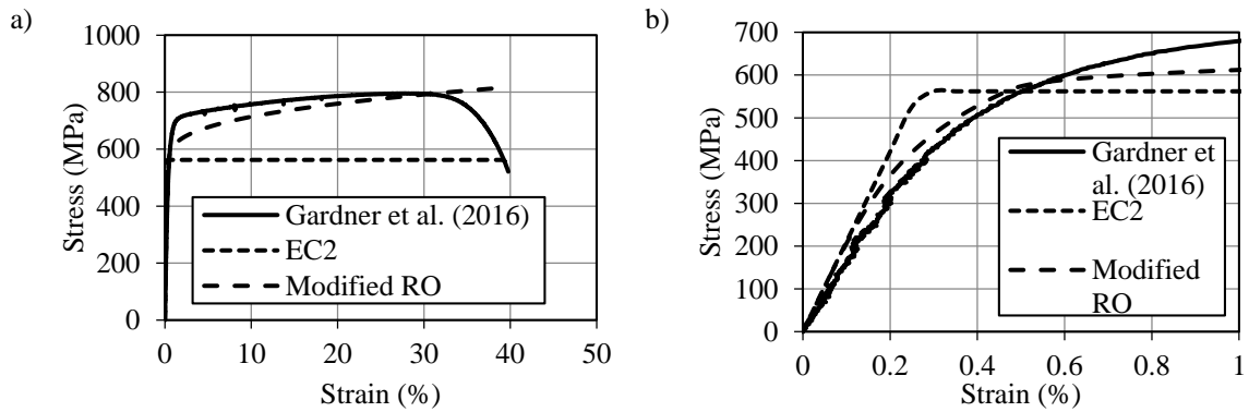
Figure 3. Experimental and design stress-strain curves for grade 1.4307 (a) full curve and (b) more detailed view of the elastic region.
