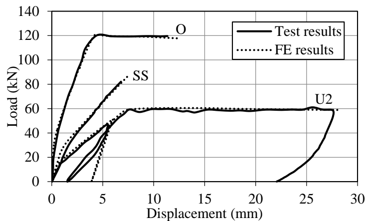
Figure 5. Comparison between the experimental and numerical load-displacement curves for beams U2, O and SS.
