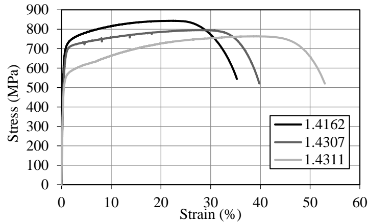
Figure 1. Stress-strain curves for different grades of stainless steel (Gardner et al., 2016).
