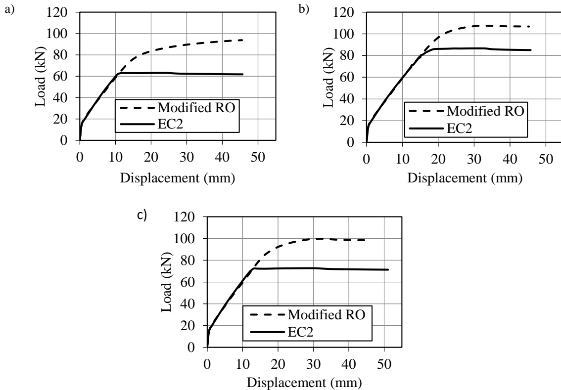
Figure 6. Influence of the stainless steel material model on the load-displacement response for beams reinforced with (a) grade 1.4311, (b) grade 1.4162 and (c) grade 1.4307 stainless steel.
