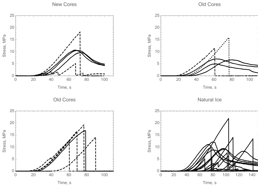
Figure 9. Stress versus the time in uniaxial compression tests with vertical ice cores. Solid, dashed and dotted lines correspond to the ice cores taken from ‘top’, ‘middle’ and ‘bottom’ layers of ice.
