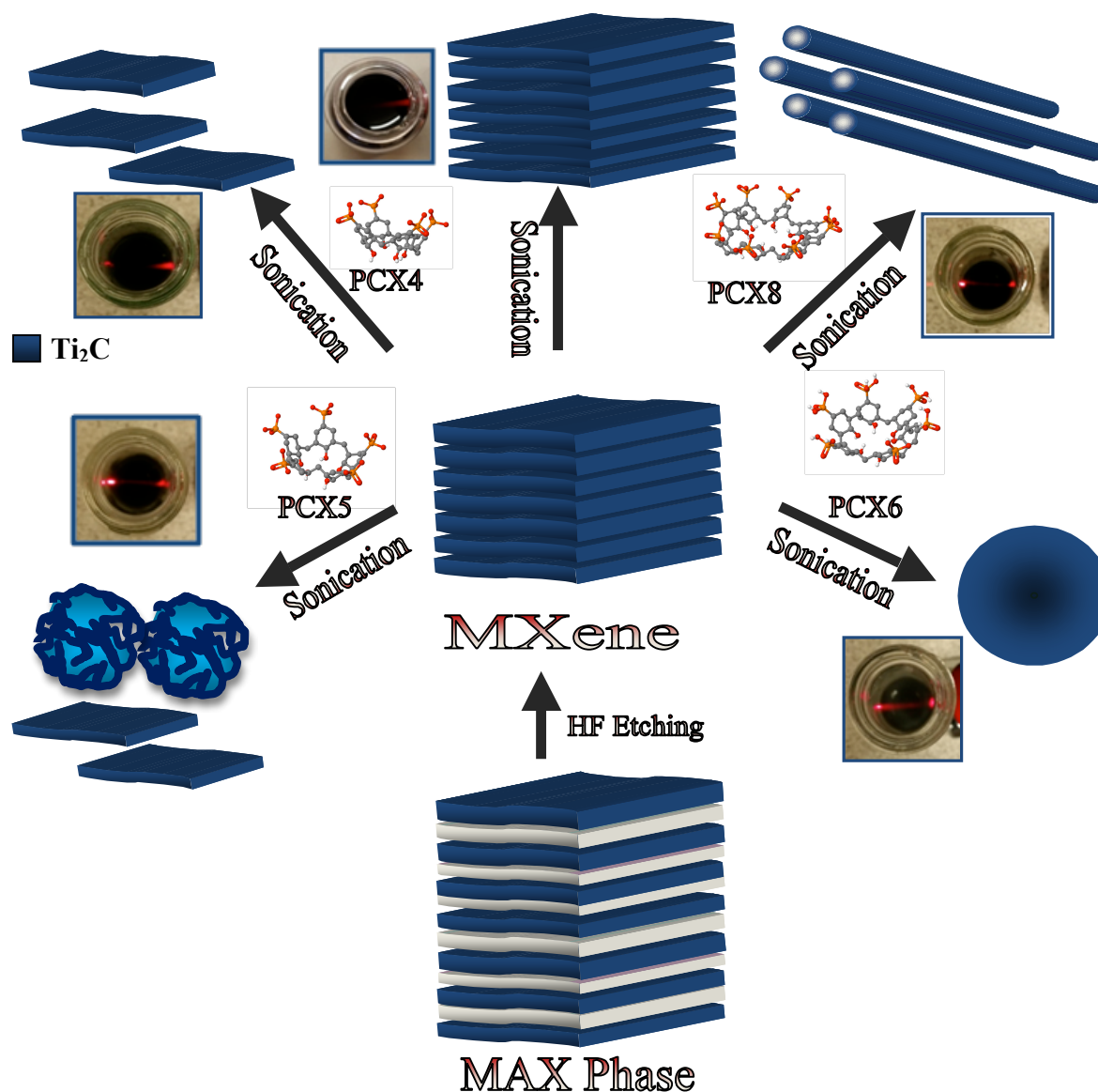
Figure 1. Schematic illustration summarizing the synthesis of different morphologies of \text{Ti}_2\text{C} . The materials were derived from HF etched MXene, mediated by ultrasonication in the presence of p -phosphonic acid calix[ n ]arenes (PCX n ). Note the Tyndall effect images for corresponding samples as confirmation of generating colloidal solution.
