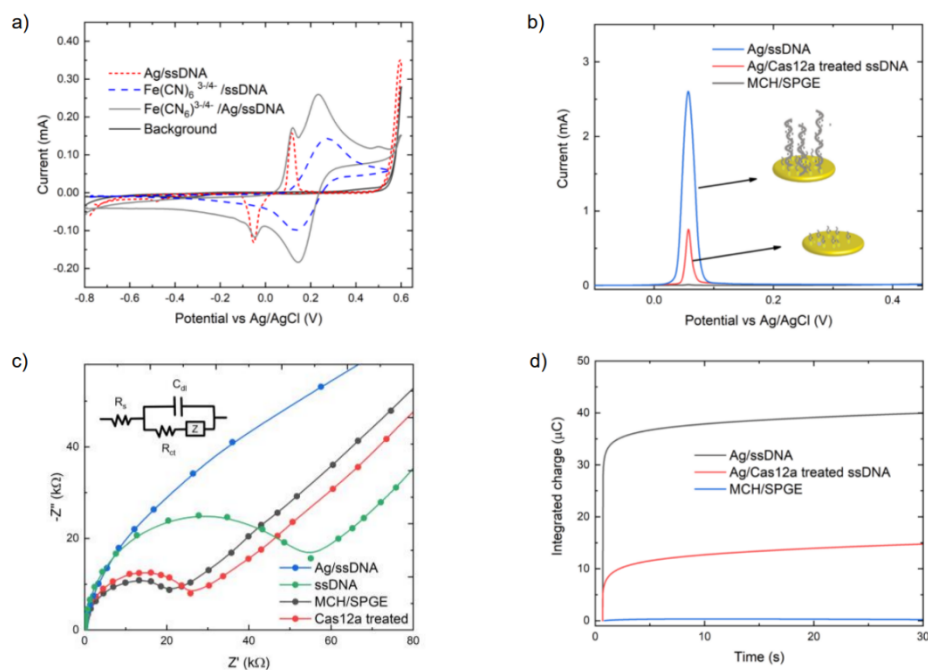
Figure 1 Comparison of MCH-modified, ssDNA-modified and Cas-treated electrodes (with 10 nM target gene) using (a) cyclic voltammetry (CV), (b) square wave voltammetry (SWV), (c) electrochemical impedance spectroscopy (EIS) and (d) controlled potential coulometry. Square wave voltammograms of silver-metallized electrodes were carried out using a step potential of 0.01 V, an amplitude of 60 mV, and a frequency of 200 Hz. For cyclic voltammograms and Nyquist plots, 10 mM [\text{Fe}(\text{CN})_6]^{3-/4-} in 0.1 M PBS was used as the working solution, and 0.1 M PBS was used as the background electrolyte. The reversible cyclic voltammograms were carried out using a scan rate of 100 mV/s, while Nyquist plots were obtained by applying a 5 mV sine wave potential within a frequency range of 10^{-2} to 10^5 Hz. For coulometry, silver was deposited using a similar protocol as SWV, then applying 0.5 V potential for 30 seconds to collect silver metallized amount on electrode.
